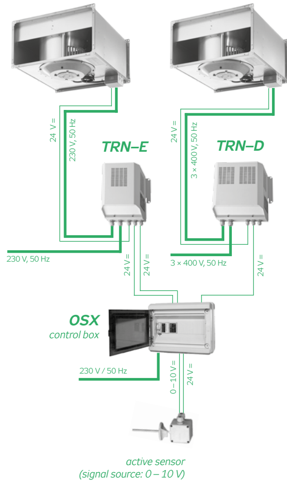
FIGURE 11 – FAN CONNECTION
