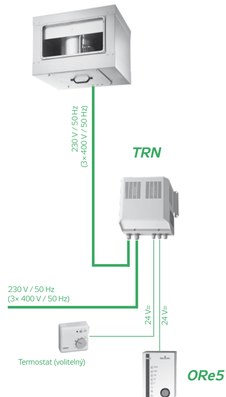
FIGURE 7 – FAN CONNECTION
