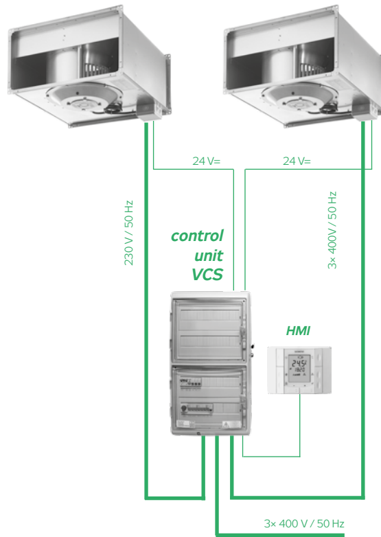
FIGURE 9 – FAN CONNECTION
