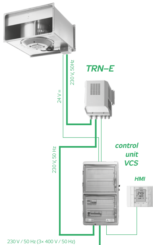
FIGURE 10 – FAN CONNECTION
